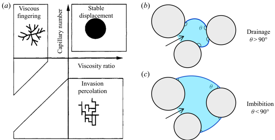
Figure 1. (a) Lenormand's phase diagram for a non-wetting fluid displacing a wetting fluid in a porous medium. The displacement front advances through either viscous fingering, stable displacement or invasion percolation, depending on the values of Ca and M . Adapted from Lenormand (1990); we endow Lenormand's phase diagram with wettability, characterized through angle \theta : (b) \theta > 90^\circ in drainage and (c) \theta < 90^\circ in imbibition.
